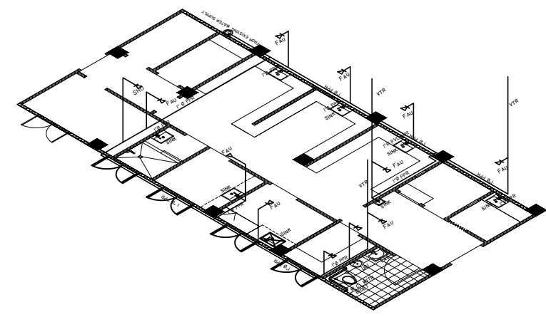
WATER LINE ISOMETRIC LAY-OUT
