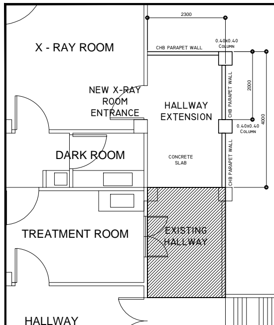
EXTENSION OF HALLWAY
