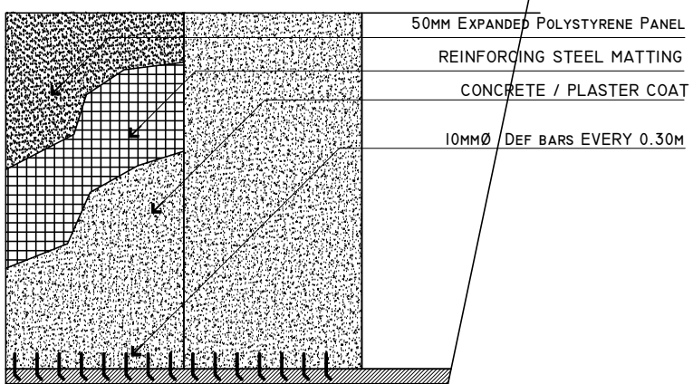
3D WALL PANEL
