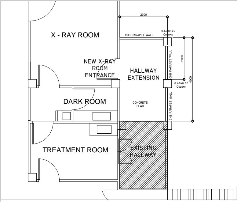
EXTENSION OF HALLWAY
