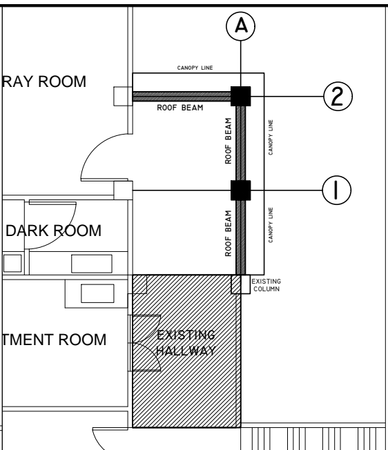
ROOF BEAM LAY-OUT
