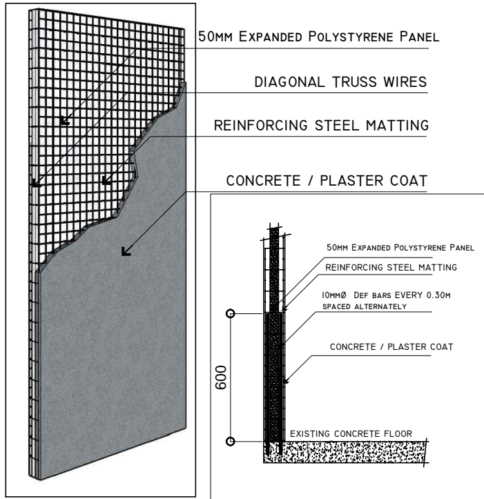
3D WALL PANEL DETAILS
