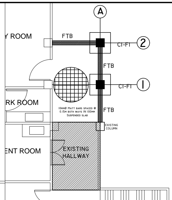
FOUNDATION LAY-OUT
