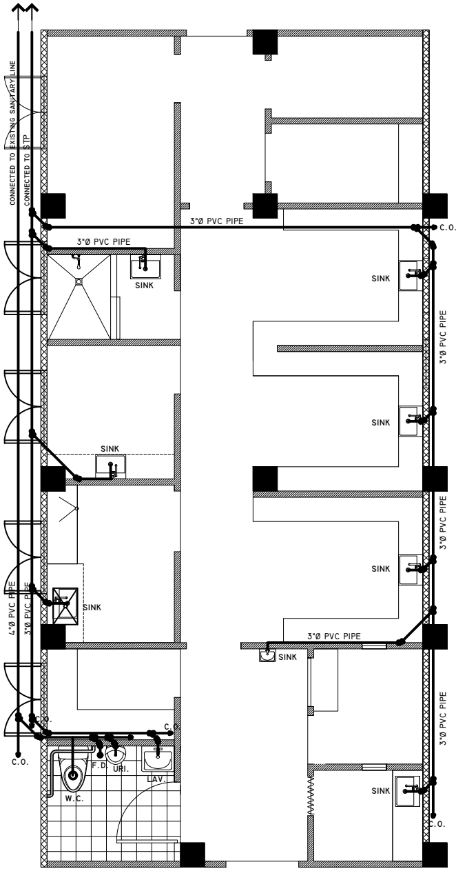
SANITARY LINE LAY-OUT
