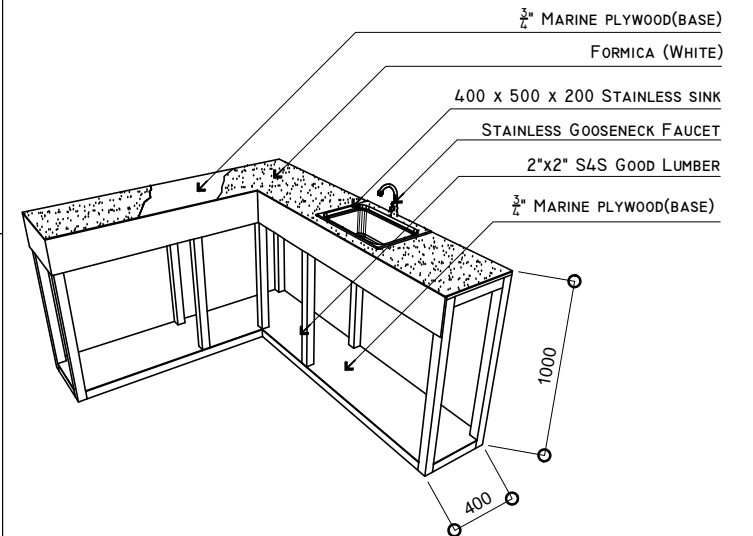
TYPICAL COUNTER WITH SINK DETAILS
