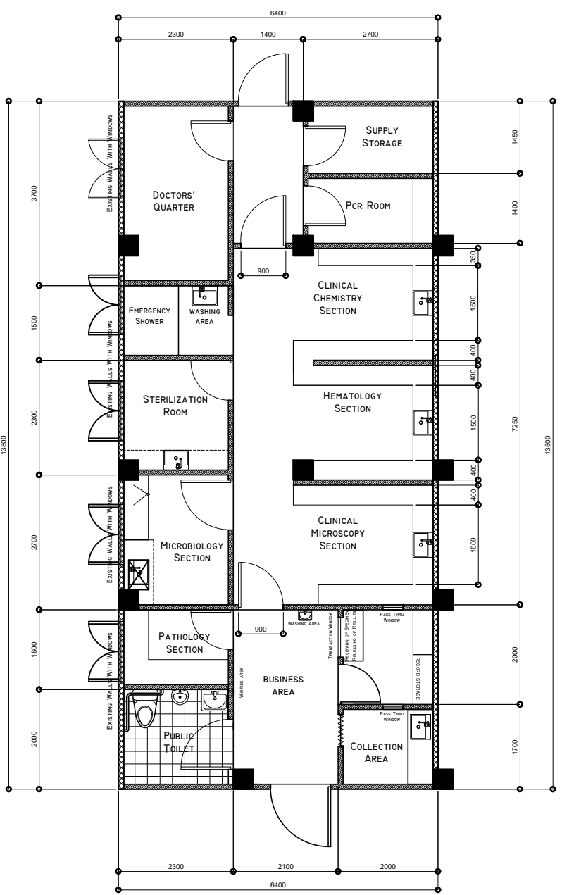
PROPOSED FLOOR PLAN
