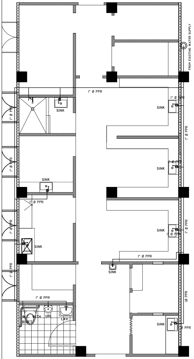
WATER LINE LAY-OUT
