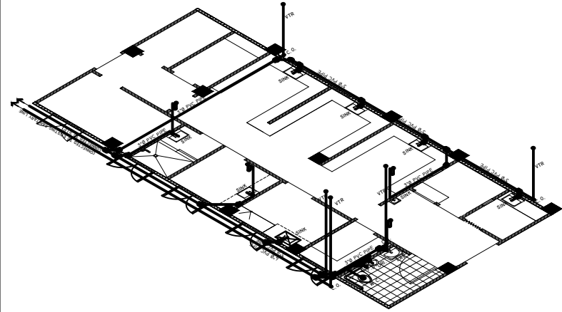
SANITARY LINE ISOMETRIC LAY-OUT
