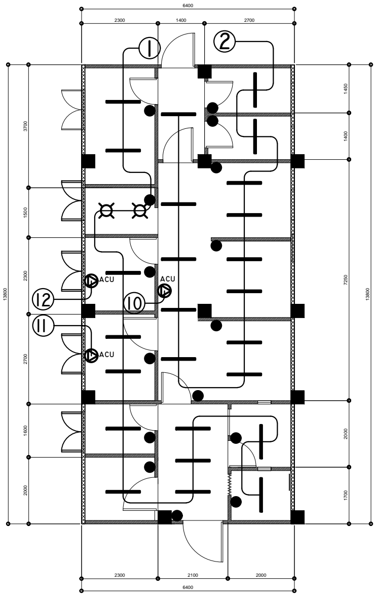
LIGHTING LAY-OUT
