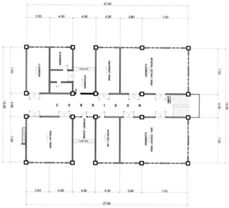
FLOOR PLAN (AREA-10) SCALE: 1:100MTRS. (GROUND FLOOR)
