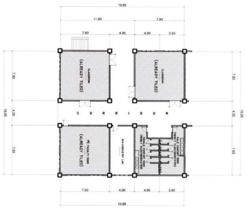
FLOOR PLAN (AREA-4) SCALE: 1/100MTS.
