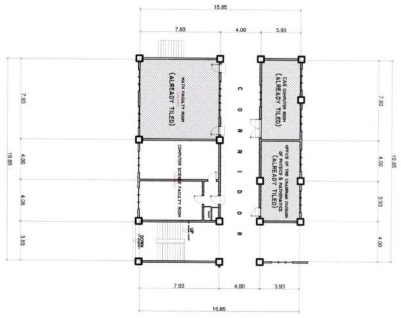
FLOOR PLAN (AREA-3) SCALE: 1/100MTS.
