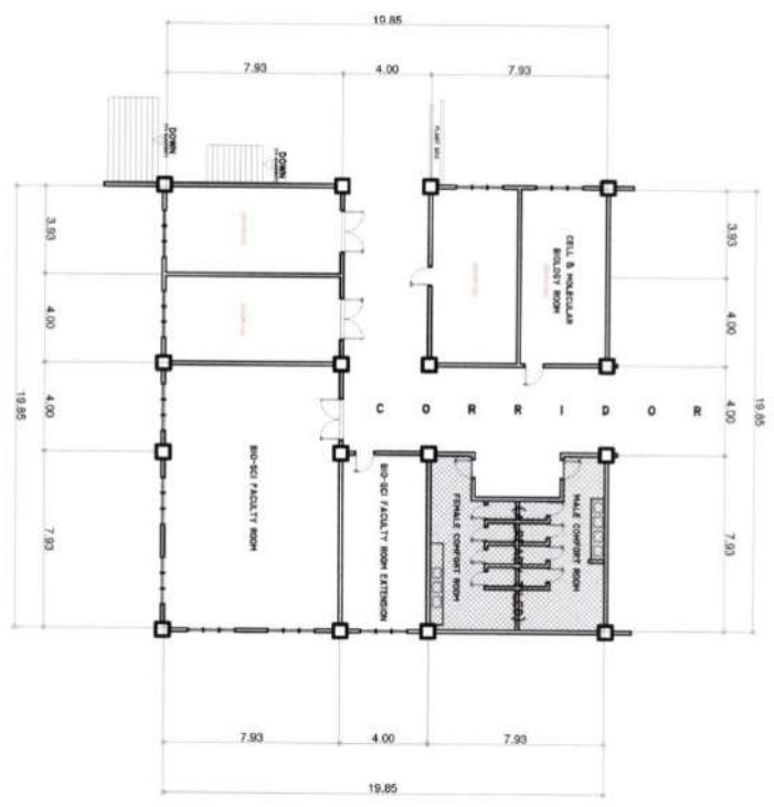
FLOOR PLAN (AREA-9) SCALE: 1:100MTRS. (GROUND FLOOR)
