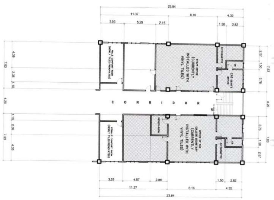
FLOOR PLAN (AREA-1) SCALE: 1/100MTS. (BASEMENT)
