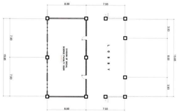
FLOOR PLAN (AREA-13) SCALE (SECOND FLOOR) 1:100M.TS.
