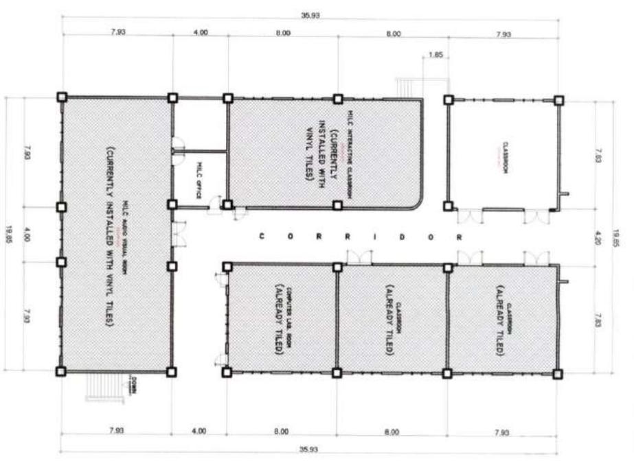
FLOOR PLAN (AREA-2) SCALE: 1/100MTS. (BASEMENT)
