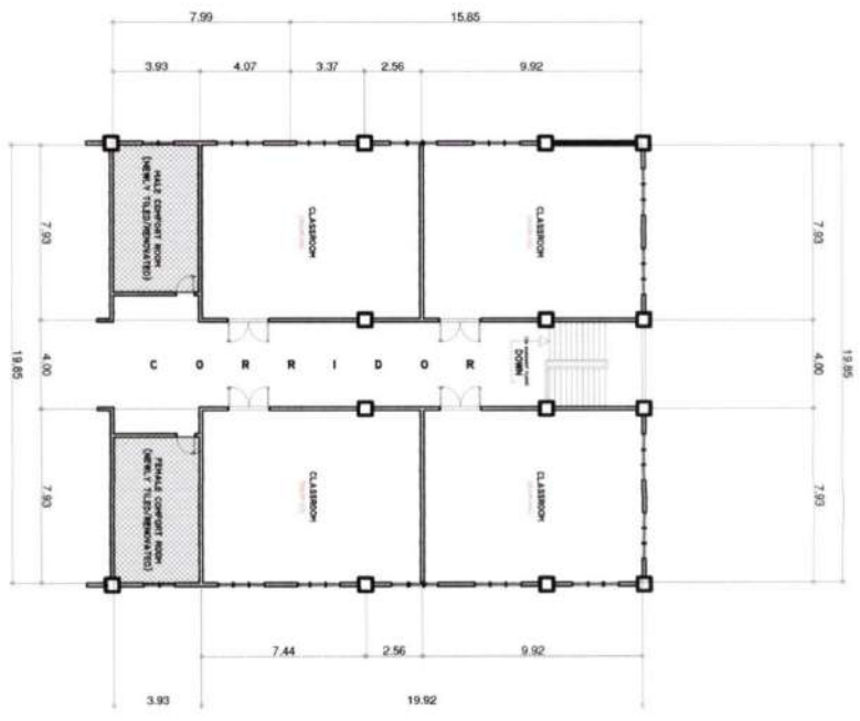
FLOOR PLAN (AREA-6) SCALE 1:100PTS. (GROUND FLOOR)
