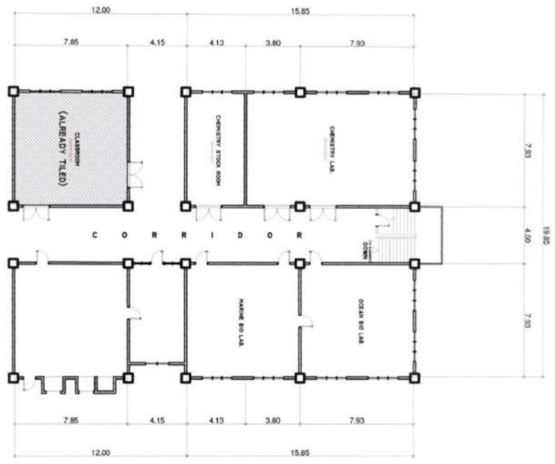
FLOOR PLAN (AREA-5) SCALE 1:100PTS. (BASEMENT)
