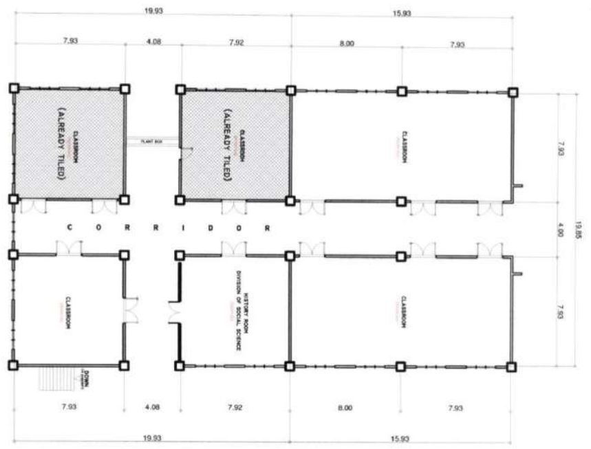
FLOOR PLAN (AREA-7) SCALE 1:100 (GROUND FLOOR)
