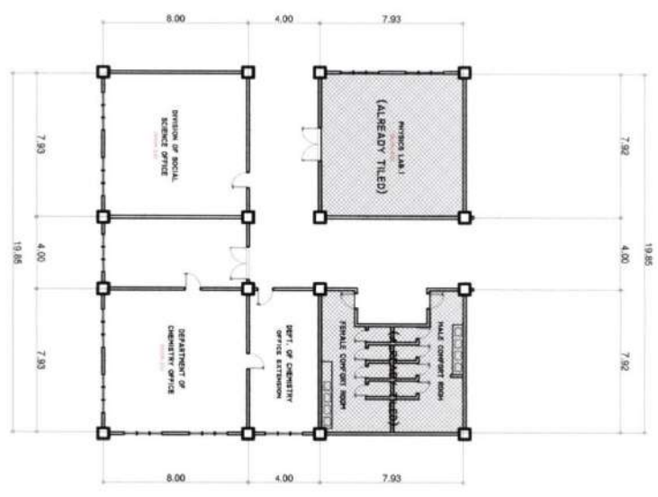
FLOOR PLAN (AREA-14) SCALE (SECOND FLOOR) 1:100M.TS.
