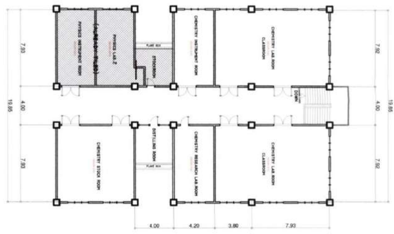
FLOOR PLAN (AREA-15) SCALE (SECOND FLOOR) 1:100M.TS.
