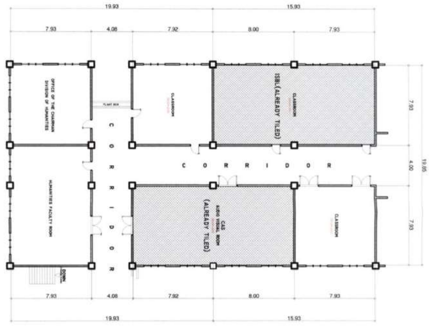
FLOOR PLAN (AREA-12) SCALE 1:100MTRS.
