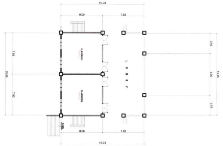
FLOOR PLAN (AREA-8) SCALE 1:100 (GROUND FLOOR)
