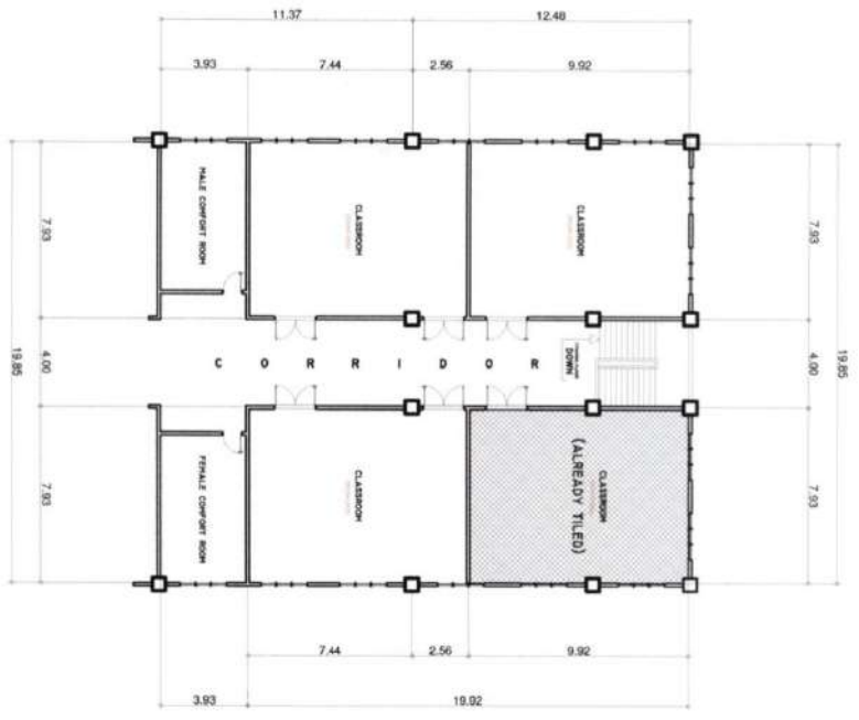
FLOOR PLAN (AREA-11) SCALE 1:100MTRS.
