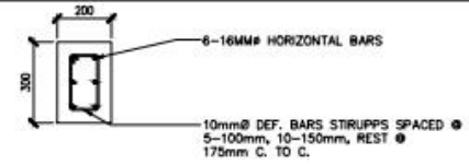
3 DETAILS OF FOOTING TIE BEAM AD-02 SCALE 1:10
