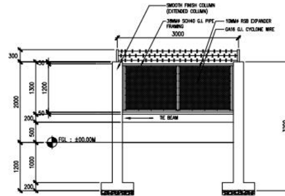
3 TYPICAL FENCE SECTION AD-02 SCALE 1:30
