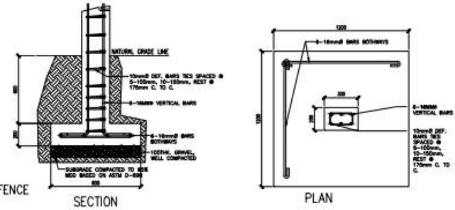
4 DETAILS OF COLUMN AND FOOTING AD-02 SCALE 1:10
